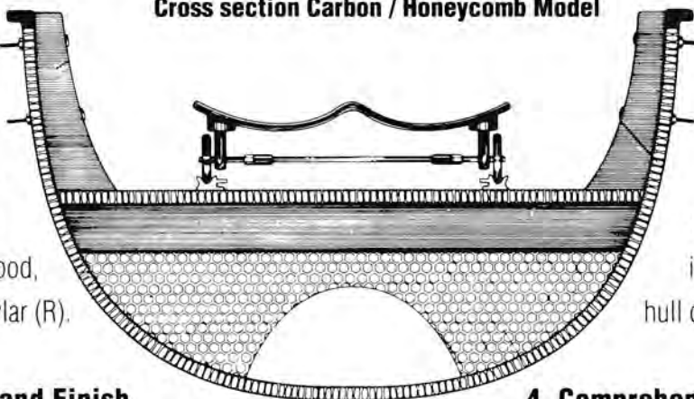
Cross section Carbon / Honeycomb Model
